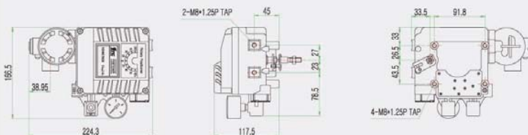
YT-1000R+L/S(ext) YT-1000R+PTM+L/S(ext)
